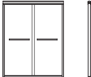
HD2501 Shower Partition 8mm tempered glass double sliding door size is custom-made
