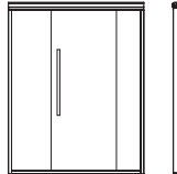
HD2502 Shower Partition 8mm tempered glass two fixed glass one sliding door size is custom-made
